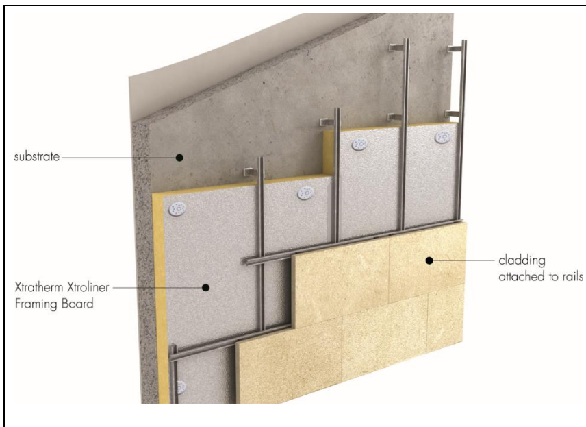
Figure 1 Example installation
